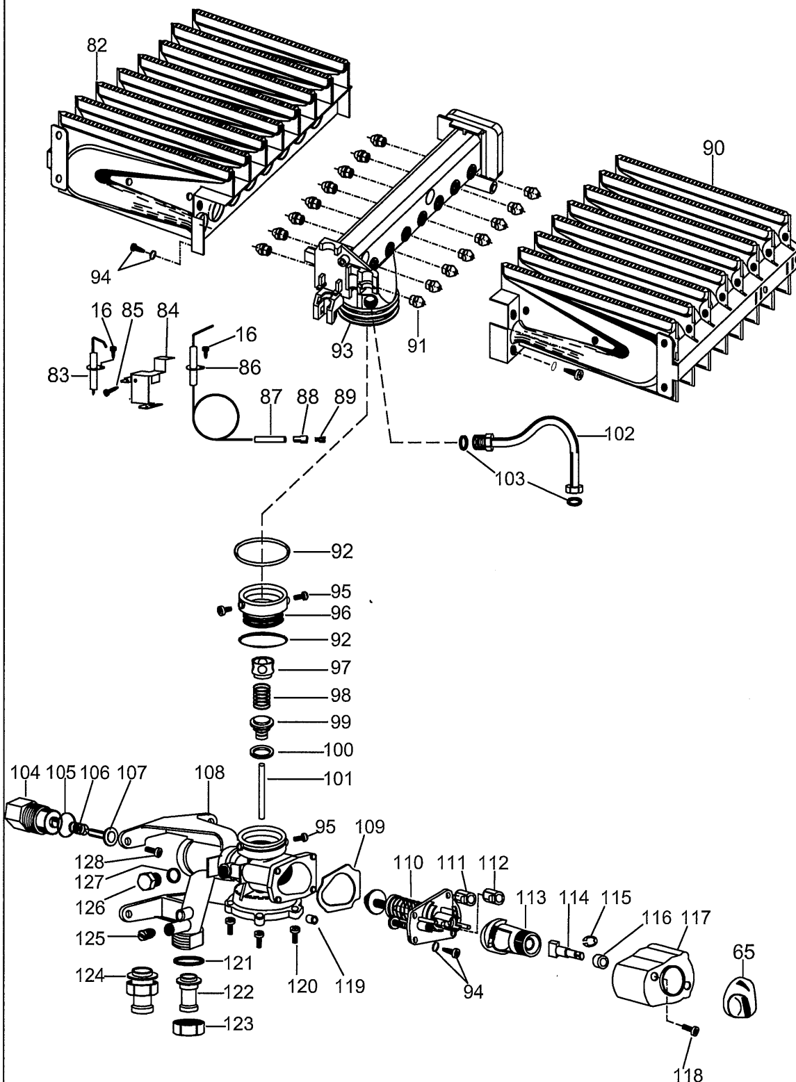
CIRCUITO GAS
